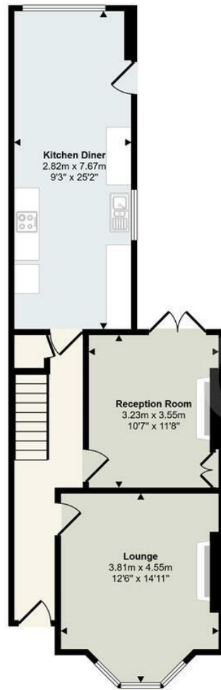
Ground Floor Approx 60 sq m / 647 sq ft
